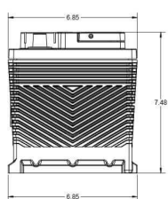
ODP-AGM48/H6/L3 RIGHT POSITIVE SAE TERMINALS
